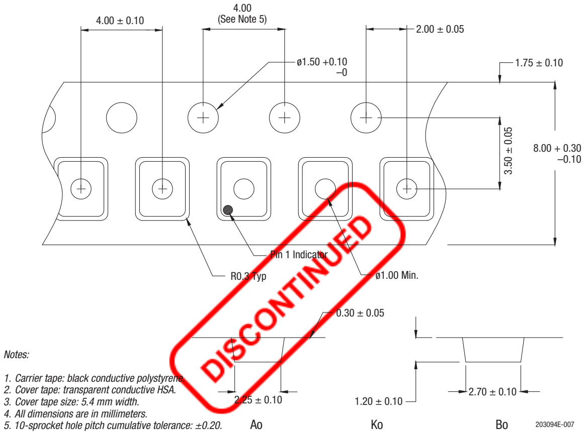
Figure 8. SKY65450-92LF Tape and Reel Dimensions
