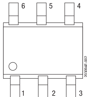
Figure 2. SKY65450-92LF Pinout (Top View)
