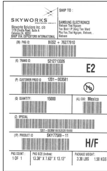
Internal Shipping Container (Samsung)
